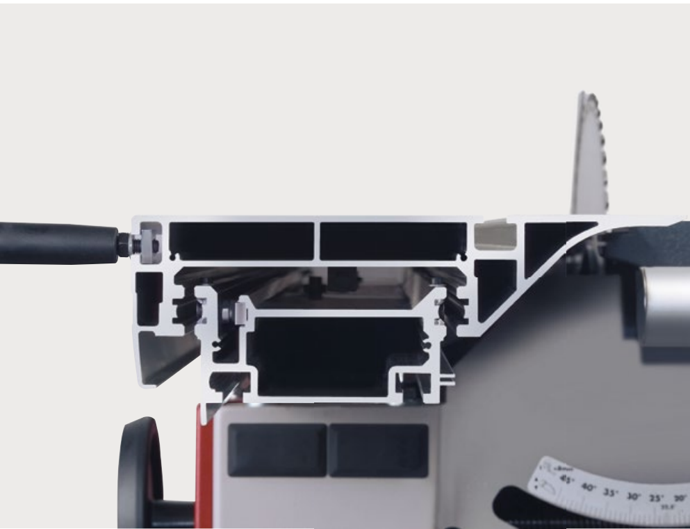
The aluminum sliding table, panel saw The aluminum sliding table gives the precision from the first cut. Guaranteed Hammer stability and precision: the strong ribbed, milled and anodised aluminum hollow-chamber profile of the sliding table in combination with the high quality guiding system ensures maximum accuracy and precision!
