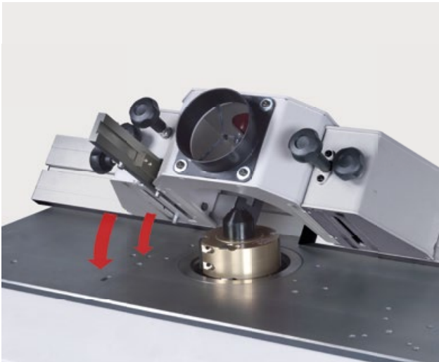
The MULTI-fine adjustment system Professional equipment: spindle fence “220” for max. tool Ø of 8.66” , MULTI adjustment system for spindle fence “220” for parallel alignment and quick adjustment.
