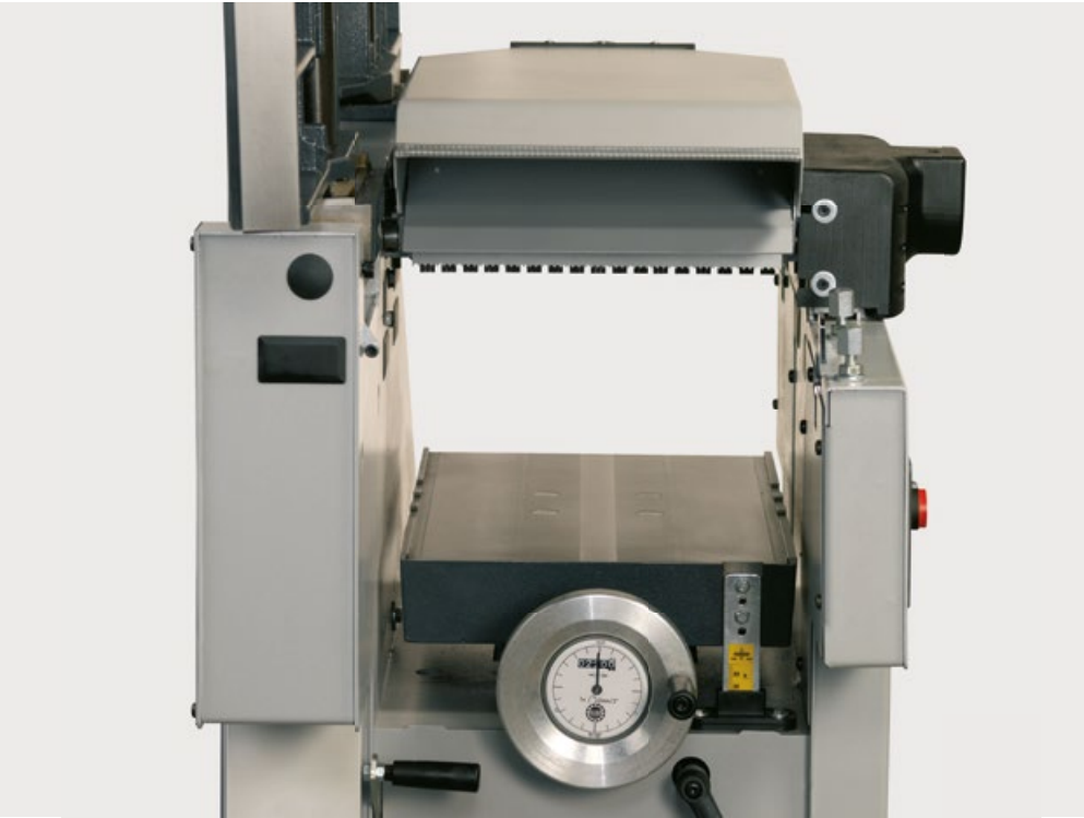
thickness planer Jointing table adjustment accurate to within a tenth of a millimeter with handwheel and integrated digital display. Max. jointing height 8 21 / 32 ".
