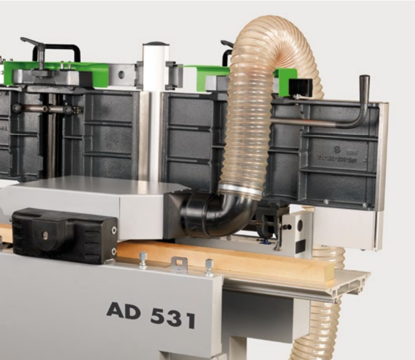
Felder table extensions Using the tried and tested FELDER table extensions it is quick and easy to extend your planing table by up to 39 3 / 8 " without the use of tools.
