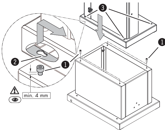
Abb. 7-3: Montage - Bandsäge
