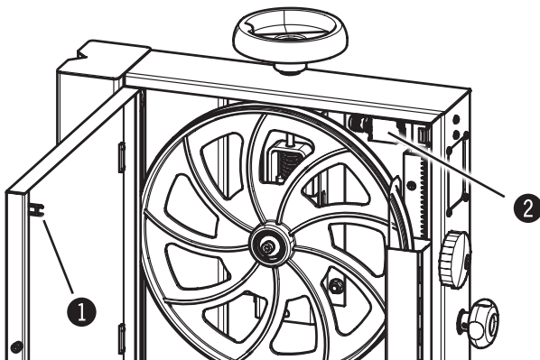
Abb. 5-3: Verriegelung
